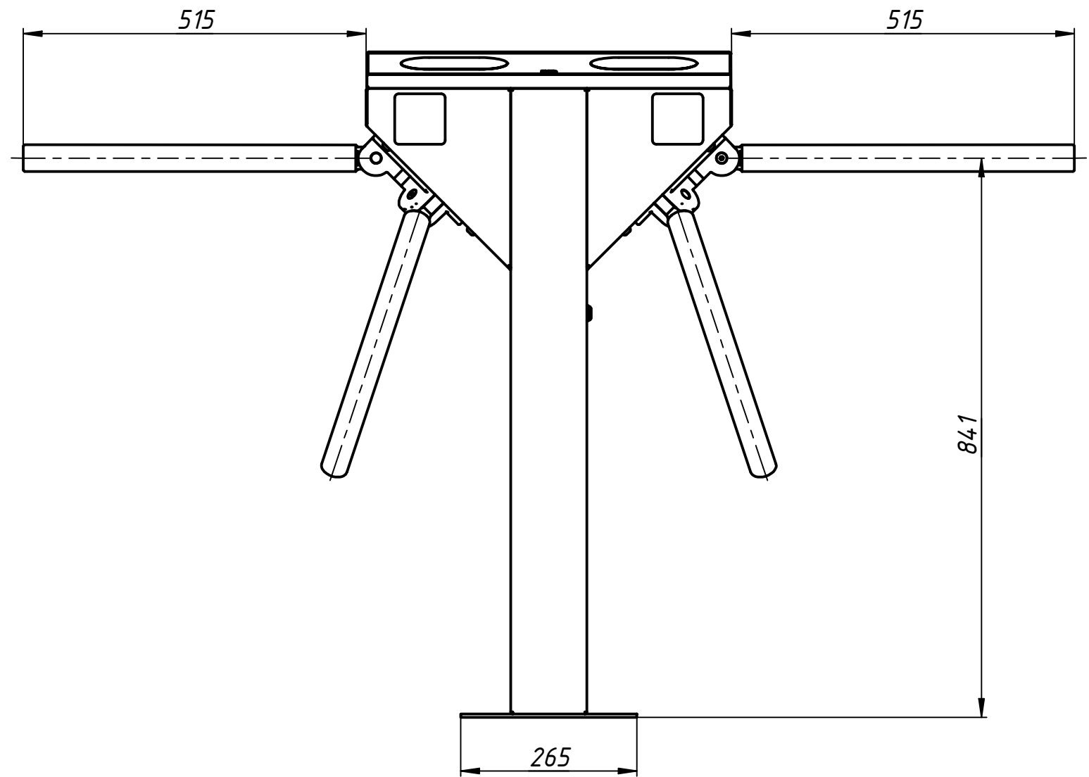
Installation tamplate
